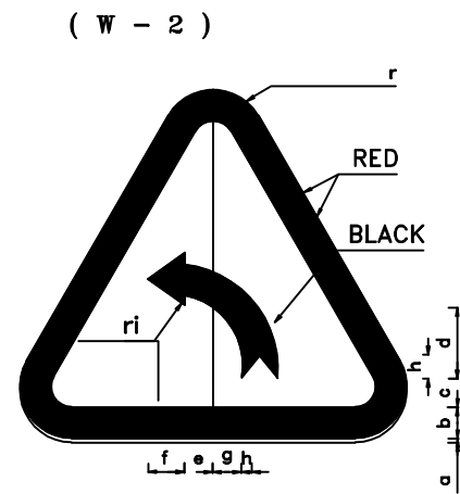
CURVE TOWARDS LEFT SIGN LEGEND DIMENSION(cm)
