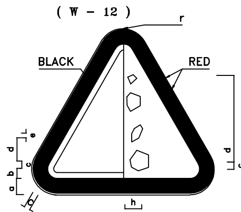
FALLING ROCK SIGN
