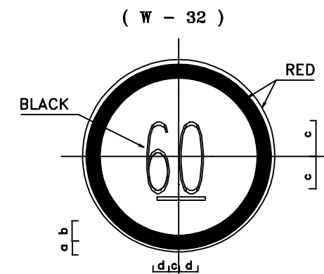
MAXIMUM SPEED LIMIT
