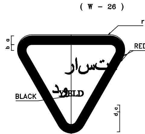
GIVE AWAY SIGN
