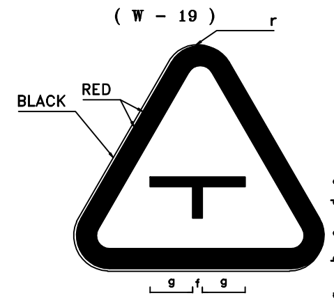
MAJOR ROAD AHEAD SIGN LEGEND DIMENSION(cm)
