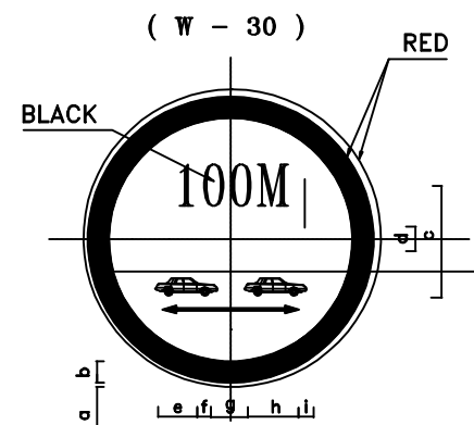
MIN.DISTANCE BETWEEN VEHICLES
