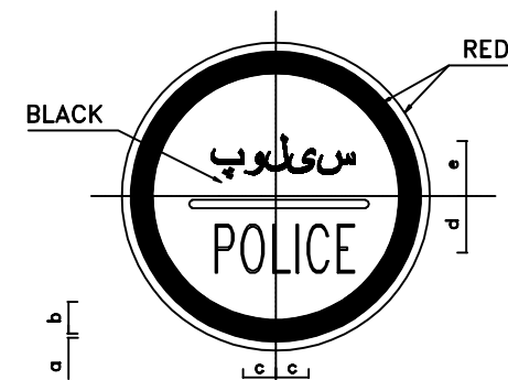
POLICE CHECK POST SIGN
