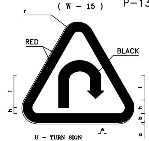
U - TURN SIGN LEGEND DIMENSION(cm)
