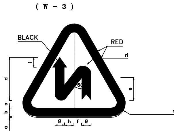
LEFT REVERSE CURVE SIGN LEGEND DIMENSION(cm)
