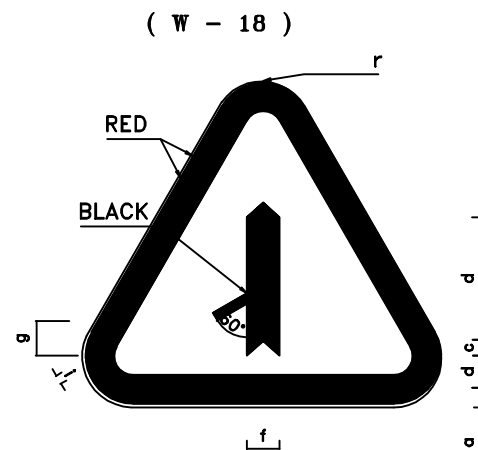
MAJOR ROAD FROM RIGHT
