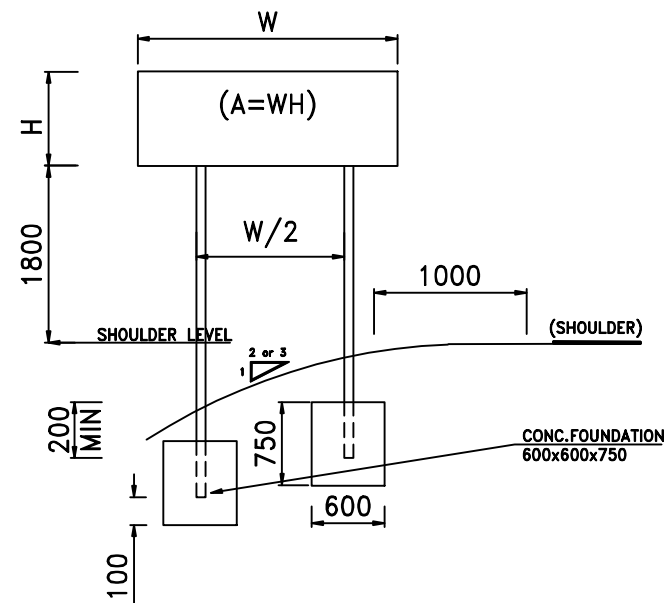
DOUBLE POST ( A \leq 3M^2 )
