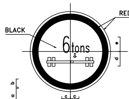
AXLE WEIGHT LIMIT SIGN
