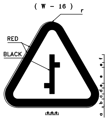
MINOR ROAD CROSSING WITH AN OFFSET LEGEND DIMENSION(cm)
