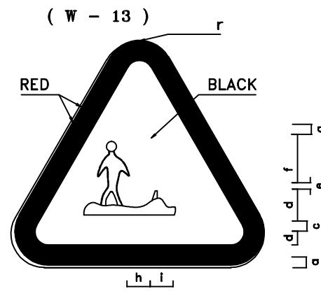
ROAD WORKS SIGN
