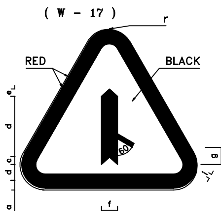
MAJOR ROAD FROM LEFT
