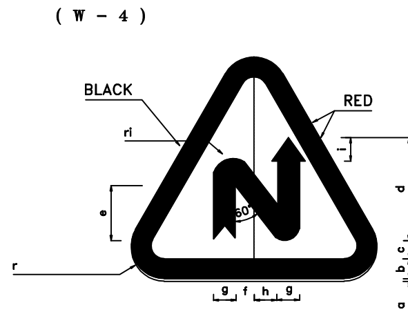
RIGHT REVERSE CURVE SIGN LEGEND DIMENSION(cm)
