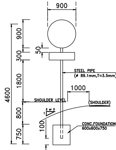
WARNING/REGULATORY (TRIANGLE/CIRCLAR)SIGNS
