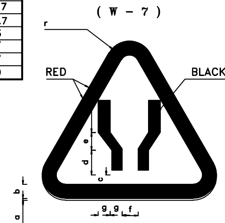
ROADWAY WIDENS SIGN LEGEND DIMENSION(cm)
