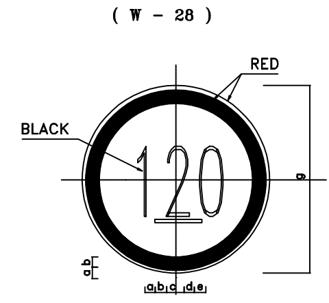
MAXIMUM SPEED LIMIT
