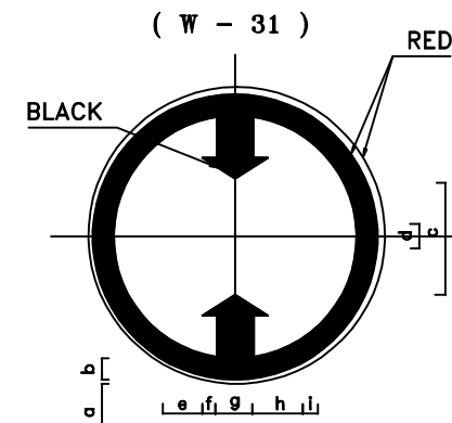
MIN.DISTANCE BETWEEN VEHICLES
