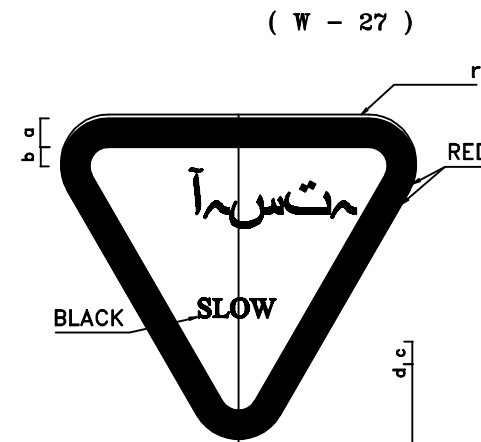
SLOW SIGN
