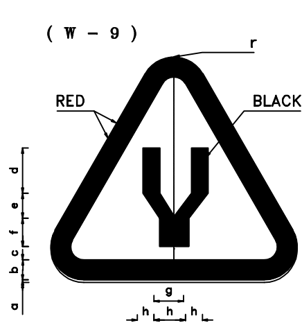
DUEL CARRIAGEWAY STARTS LEGEND DIMENSION(cm)
