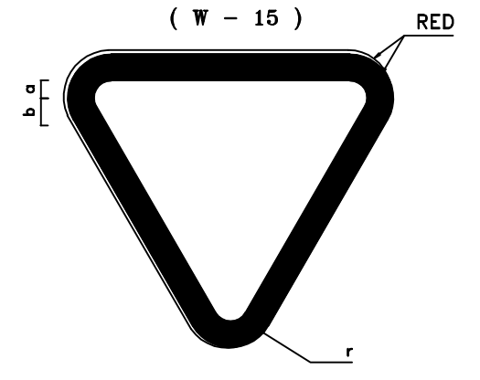
GIVE WAY SIGN
