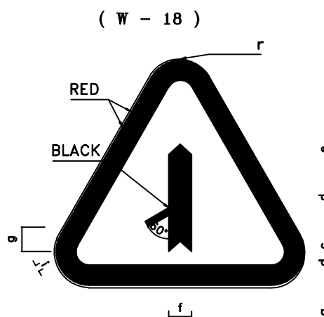
MERGE SIGN LEGEND DIMENSION(cm)
