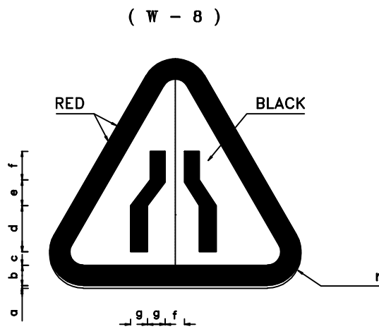
ROADWAY NARROWS SIGN LEGEND DIMENSION(cm)
