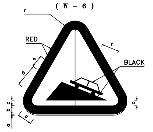
ROADWAY GRADE SIGN LEGEND DIMENSION(cm)
