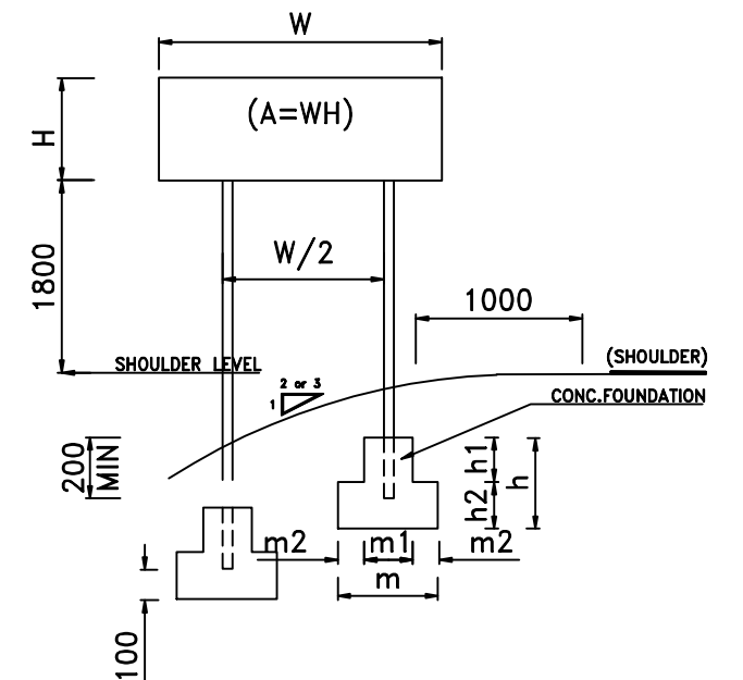
DOUBLE POST ( A > 3M^2 )
