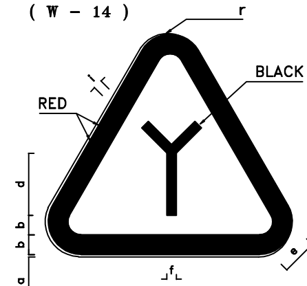
JUNCTION SIGN LEGEND DIMENSION(cm)
