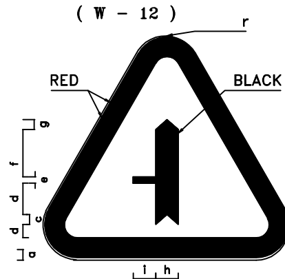
MINOR ROAD FROM LEFT LEGEND DIMENSION(cm)
