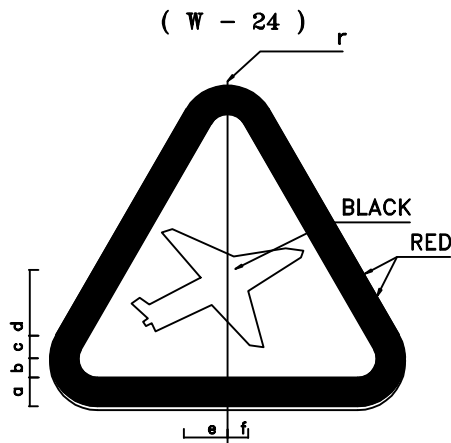
LOW FLYING AIRPORT SIGN
