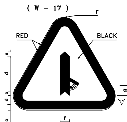
MERGE SIGN LEGEND DIMENSION(cm)
