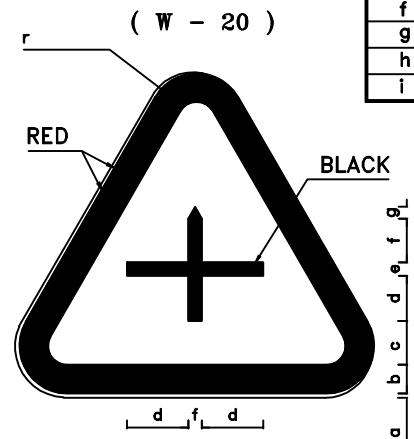
MAJOR ROAD AHEAD SIGN LEGEND DIMENSION(cm)
