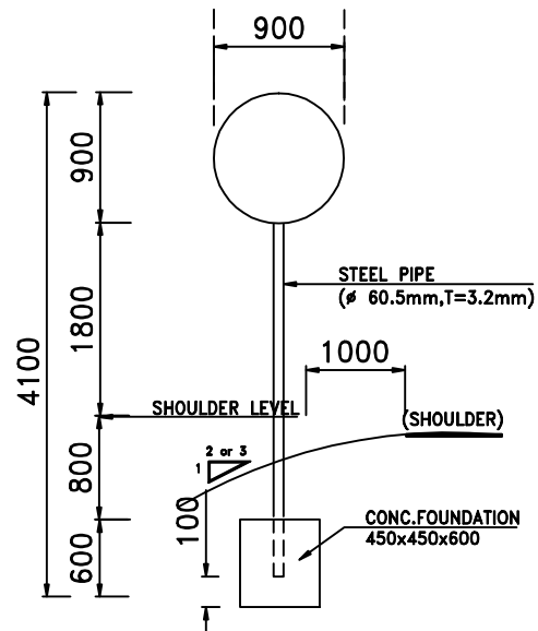
SINGLE SIGNS
