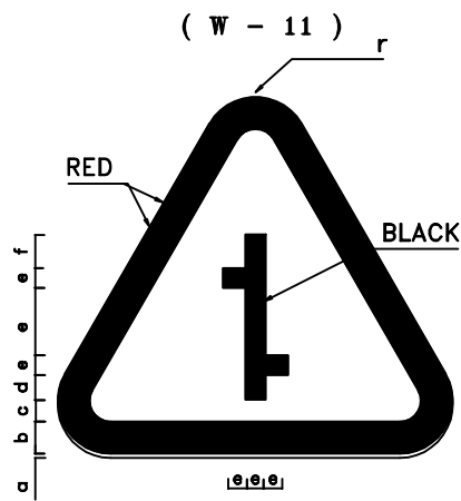
MINOR ROAD CROSSING WITH AN OFFSET LEGEND DIMENSION(cm)
