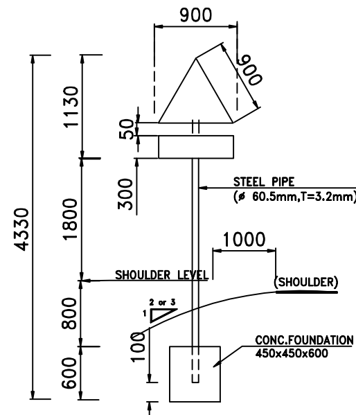
DOUBLE SIGNS
