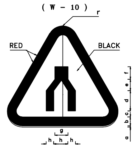
DUEL CARRIAGEWAY END LEGEND DIMENSION(cm)
