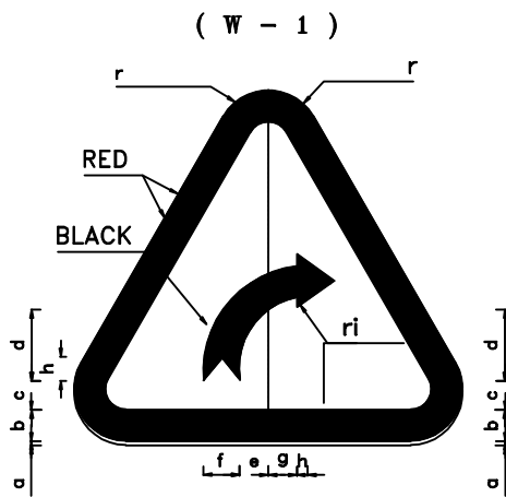
CURVE TOWARDS RIGHT SIGN LEGEND DIMENSION(cm)
